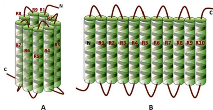
Figure 10. Two proposed three-dimensional structures of \alpha -zein: Cylindrical model (A) and ribbon-like model (B). Reproduced with permission from Zhang et al. [101].
