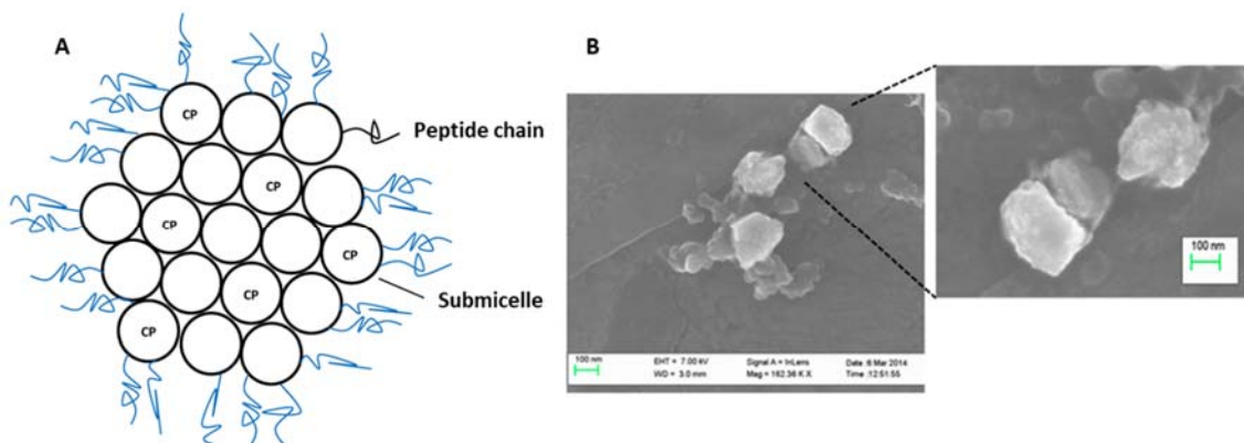
Figure 9. The structural arrangement of casein micelles. CP-Calcium phosphate (A). Reproduced with permission from Pereira et al. [92]. Scanning Electron Microscopy microphotographs of casein nanoparticles (B). Reproduced with permission from Peñalva et al. [87].
