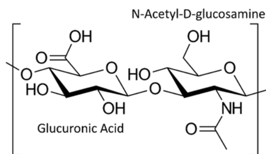
Figure 3. An image of the repeating unit of hyaluronic acid (HA).
