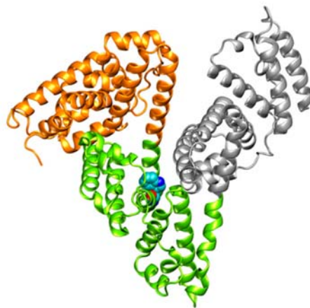
Figure 6. Crystallographic structure of HSA (PDB: 1N5U), presenting the three structurally similar domains: I (Brown), II (green), and III (grey). Reproduced with permission from Chaves et al. [76].
