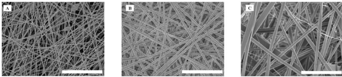
Figure 12. Scanning Electron Microscopy images of silk fibroin scaffolds obtained using different electrospinning concentrations: 7 wt % (A), 8 wt % (B) and 9 wt % (C). Scale bars: 10 \mu m. Reproduced with permission from Chen et al. [131].
