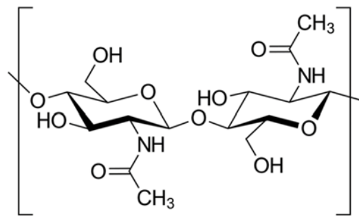
Figure 4. An image of the chemical structure of chitin.
