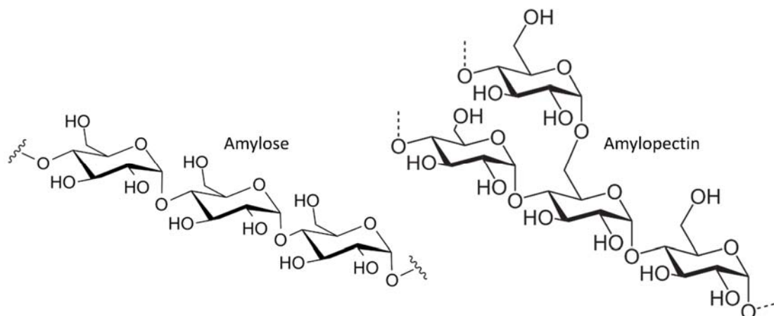
Figure 2. Chemical structure of starch detailing both amylose and amylopectin subunits.
