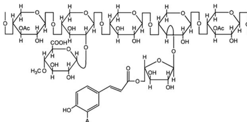
Figure 5. A representative structure of hemicellulose. Reproduced with permission from Terzopoulou et al. [72].
