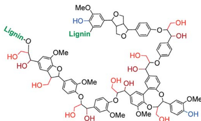
Figure 11. The proposed structure of lignin. Reproduced with permission of Dabral et al. [114].
