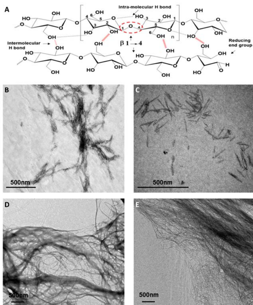
Figure 1. Cellulose structure and intra/intermolecular hydrogen bonding pattern (A). Morphological and structural characteristics of the unmodified and oxidised nanocellulose samples: Transmission electron micrographs of cellulose nanocrystals (B), oxidised cellulose nanocrystals (C), cellulose nanofibers (D) and oxidised cellulose nanofibers (E). Reprinted with permission from Tayeb et al. [30] and Siqueira et al. [31].
