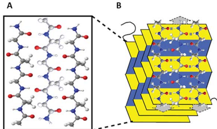
Figure 8. An image of a three-chain silk sequence composed of carbon (grey), nitrogen (blue), oxygen (red) and hydrogen (white) (A), and a 3-dimensional \beta -sheet of silk (B). Reproduced with permission from Cebe et al. [82] and Stewart et al. [83].
